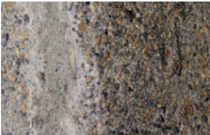
Fig. 8.7.5: Due to continuous exposure, the cement film is eroded in an initial step, and thereafter larger and larger aggregates are rubbed, knocked or washed out of the hardened cement paste.
